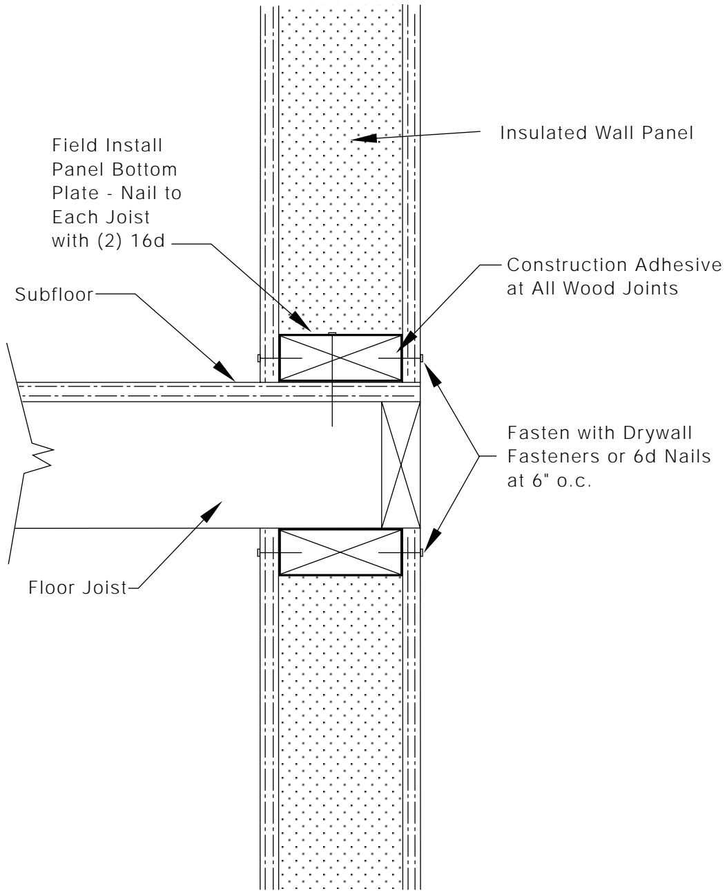
SECTION VIEW
